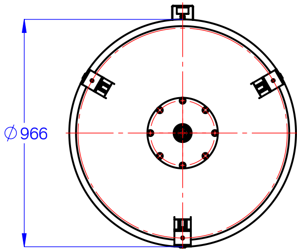
VIEW B
