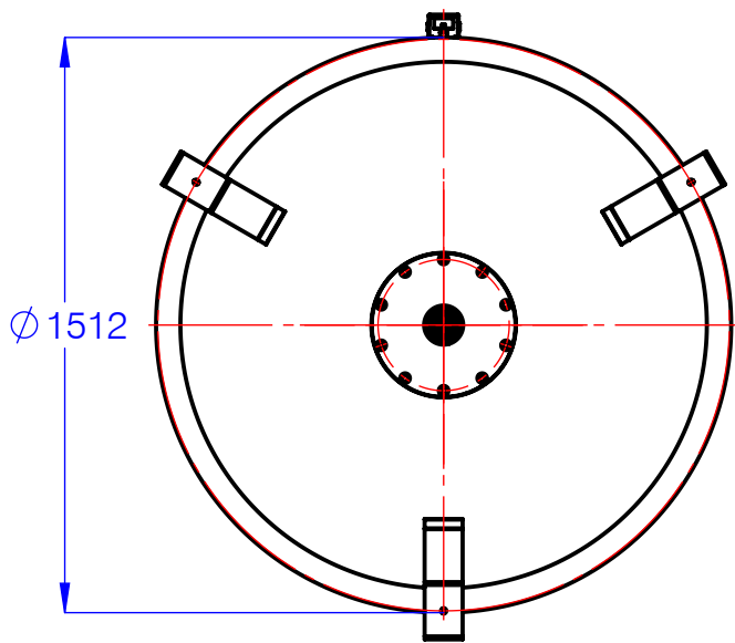
VIEW B
